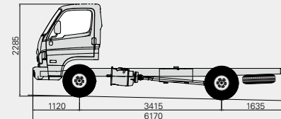
Standard Cab Medium Wheelbase
