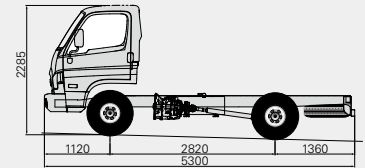
Standard Cab Short Wheelbase
