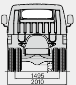
Standard Cab
