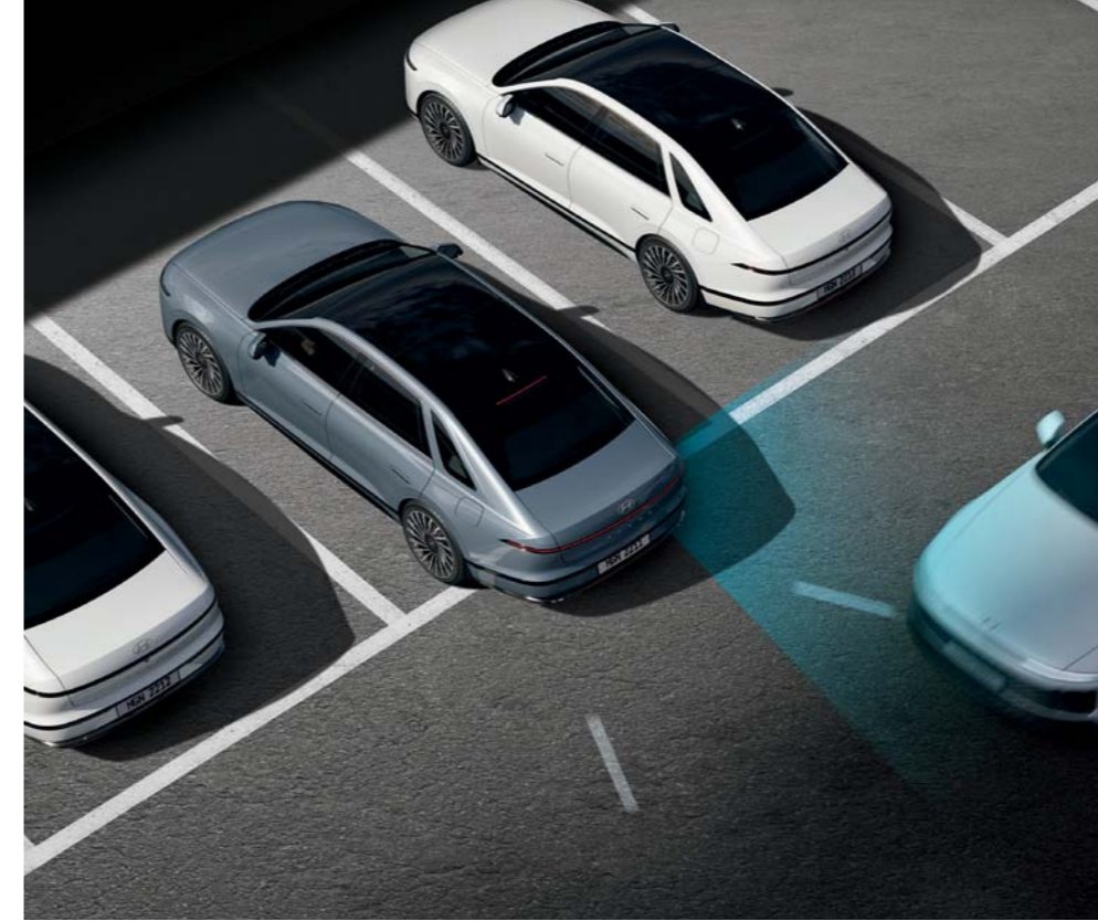
Rear Cross-Traffic Collision-Avoidance Assist (RCCA) Rear Cross-Traffic Collision-Avoidance Assist (RCCA) provides a warning if there is a risk of collision with an oncoming vehicle on the left or right side while reversing. After the warning, it automatically assists with emergency braking if the risk of collision increases.
