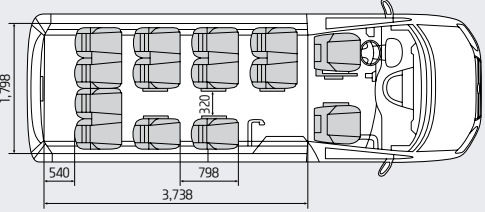
Seats for 13+1 (Front & Middle doors)
