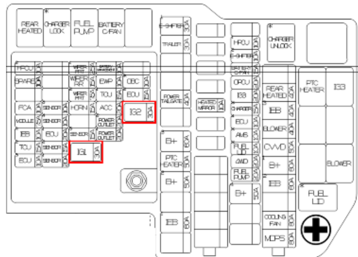
Engine room fuse box
