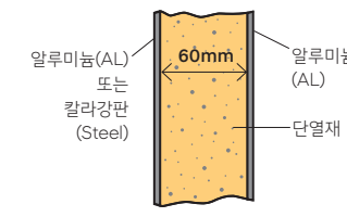
보온판넬 (A60A, A60S)
