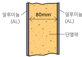
특수보온패널 (A80A) ※SIDE : A80A/FLOOR, ROOF FRONT : A80A
