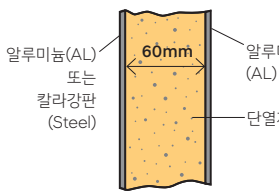
보온패널 (A60A, A60S)
